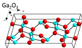
Quantum disorder
