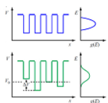
Quantum disorder
